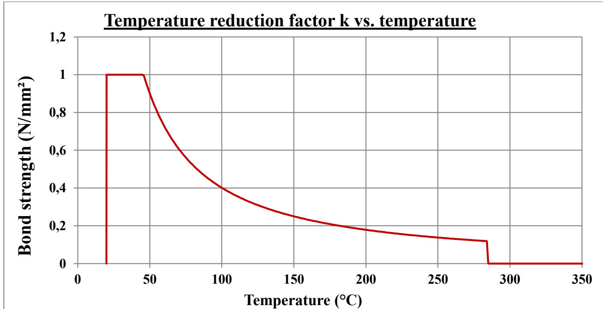
Figure 3 : Temperature reduction factor k(\theta) vs. temperature
