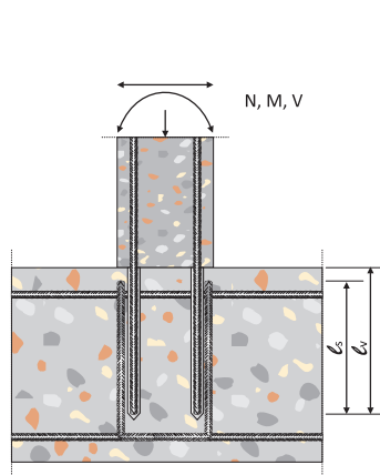
Figure 2: Overlap joint at a foundation of a column or wall where the rebars are stressed in tension
